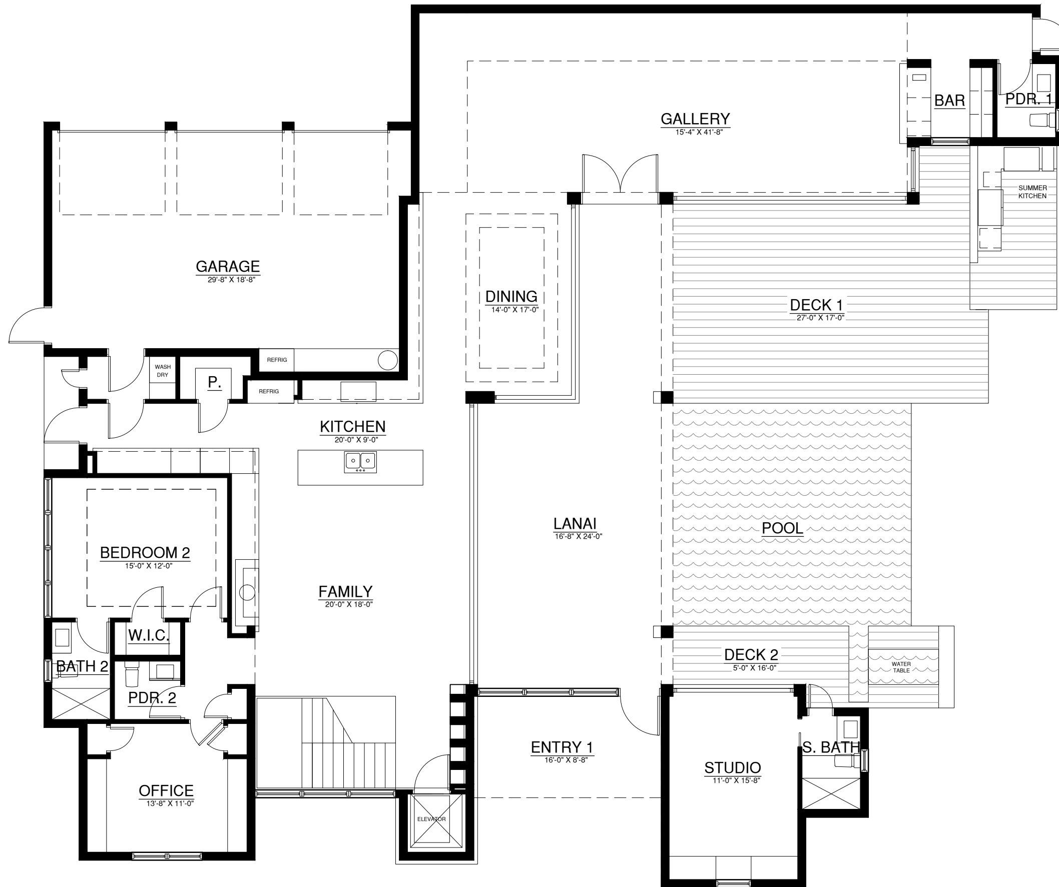
MAIN LEVEL FLOOR PLAN
