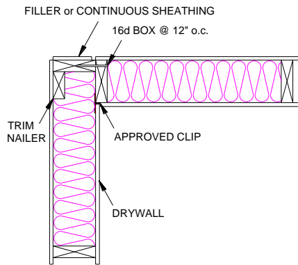
2-Stud Corner Using Drywall Clip and Exterior Nailer
