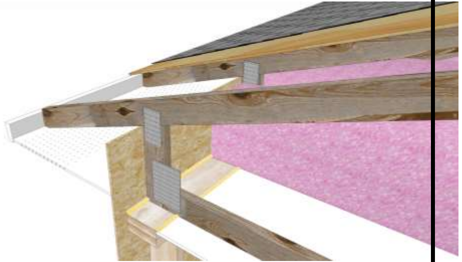
Figure 21. High Heel Truss
