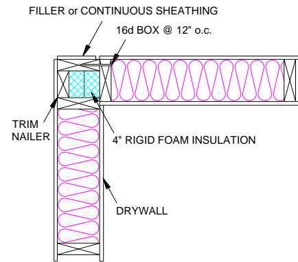
3-Stud Corner Using Exterior Nailer and Field Installed Rigid Foam
