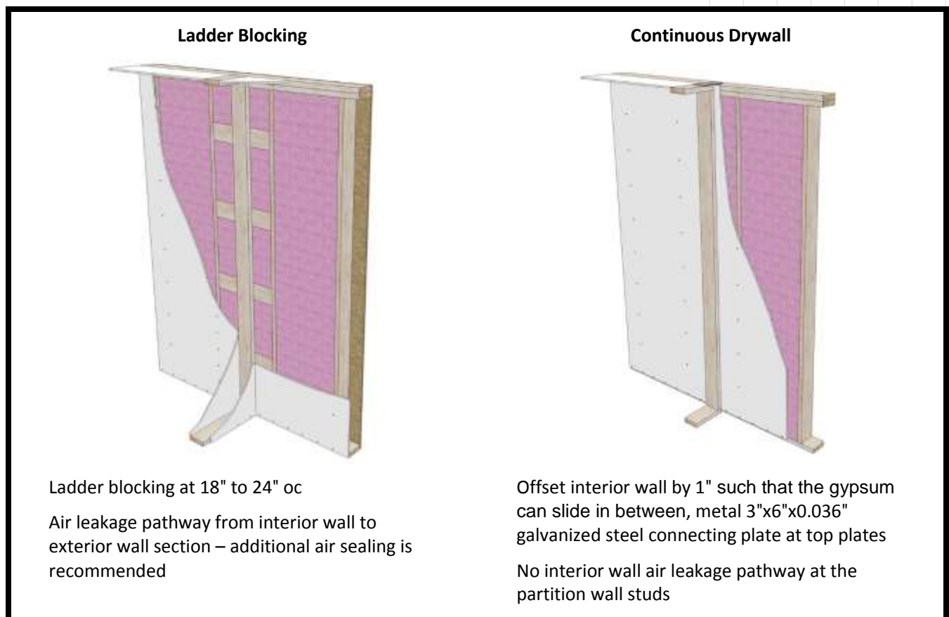
Figure 5. Advanced Framing Details for Intersecting Walls
