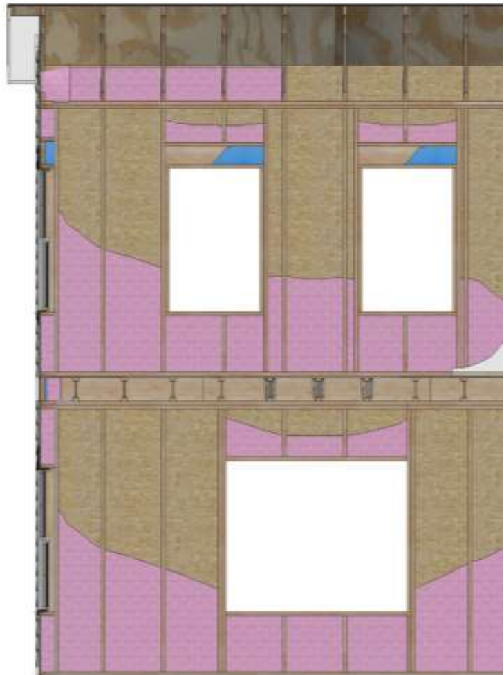
Figure 13. 1st Floor Rim and 2nd Floor Single Headers
