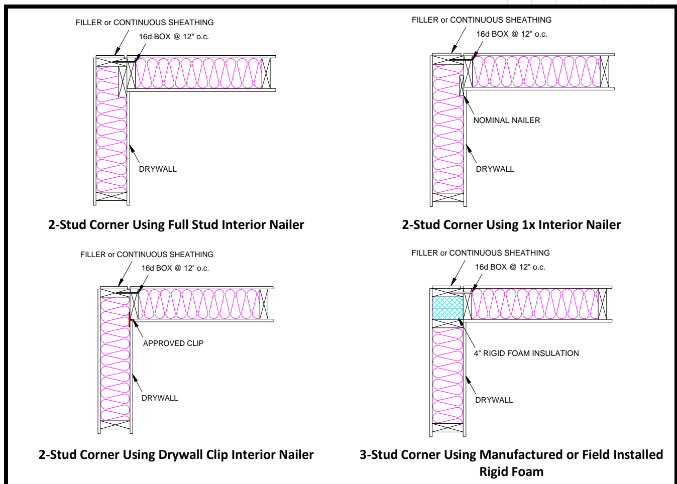
Figure 2. Corner Framing Details for Cladding Systems That Do Not Require Additional Framing for Trim
