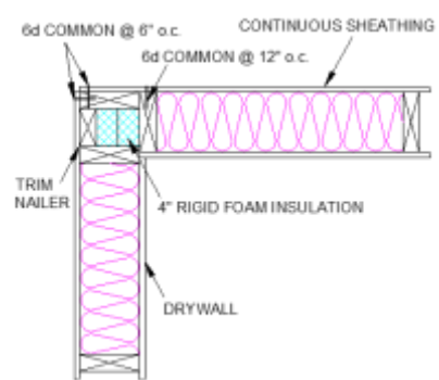
Figure 4. Continuous Sheathing Option Examples
